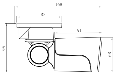
ceiling mount
